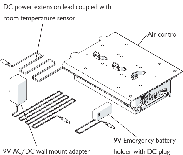
Fig. 19 Power connections
