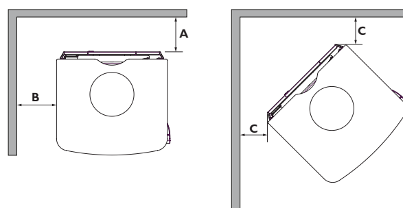
Fig. 6. Distances to combustible materials
