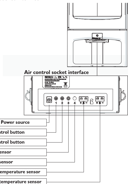
Fig. 18 Socket interface
